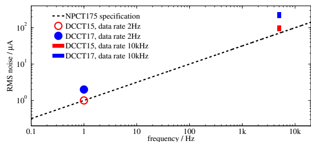
Figure 5: Amplitudes of the narrowband noise are approximately proportional to the beam current in both DCCTs.
