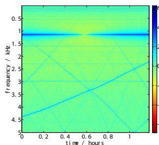
Figure 3: Waterfall plot of the spectrum of the DCCT.
