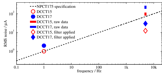
Figure 8: The resolution has a great improvement after using the adaptive notch filter.
