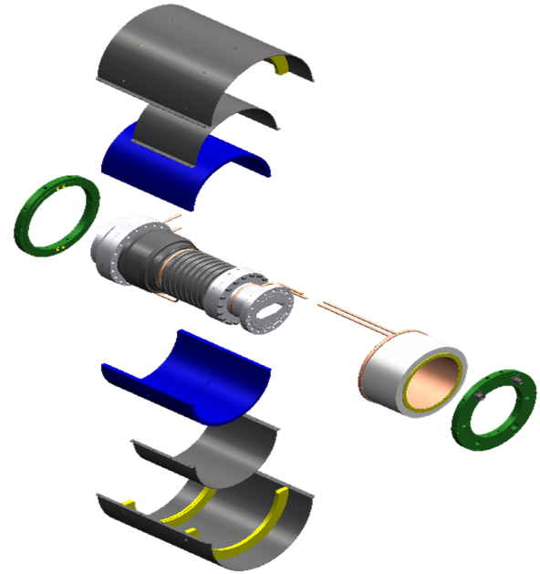
Figure 1: Exploded view of the shielding system designed by SPEAR3.
