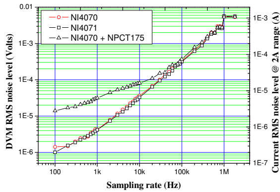
Figure 2: Noise test result of DVM and NPCT.
