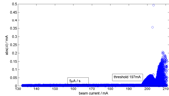
Figure 7: The square wave noise has a threshold and an interesting distribution.
