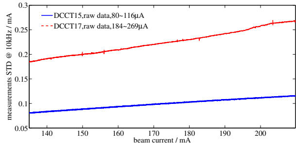
Figure 4: Amplitudes of the narrowband noise are approximately proportional to the beam current in both DCCTs.
