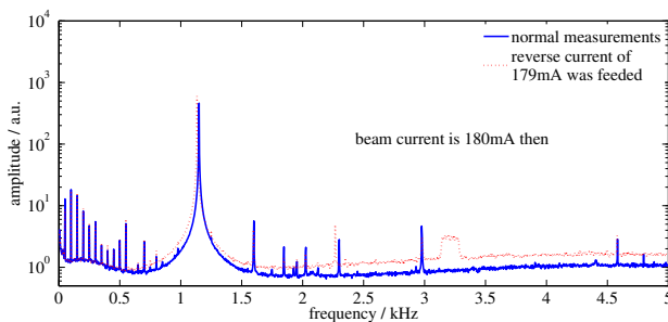
Figure 6: Comparison of the spectra.
