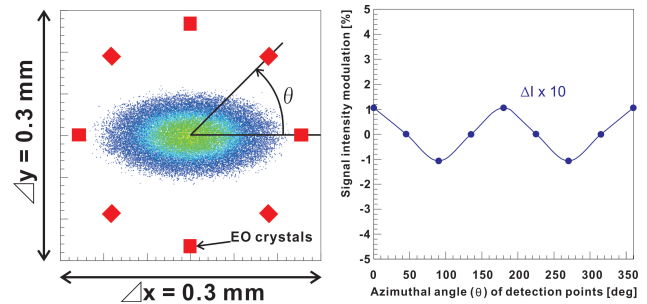
Figure 4: Longitudinally sliced BCD profile with relative coordinates of eight Pockels EO crystals ( left ) and calculation results of signal intensity modulations at each crystal position ( right ).
