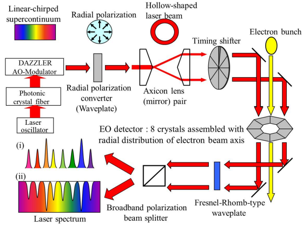
Details of EO detectors in 3D-BCD monitor
