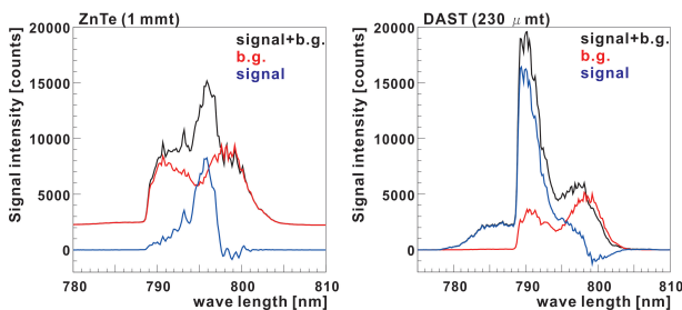
Figure 7: Signal intensity spectra of BCD measurement via 1 mm thick ZnTe (left) and 230 \mu m thick DAST (right) Pockels EO crystals. Average bunch charge is fixed as 0.28 nC.
