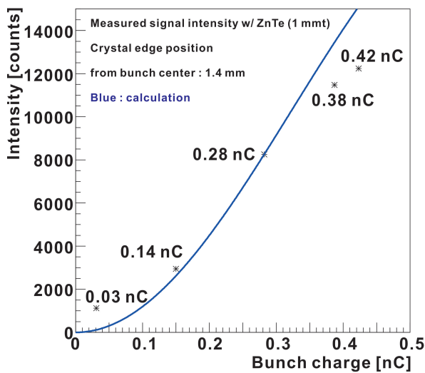
Figure 6: Dependency of the EO signal intensities on the bunch charge.
