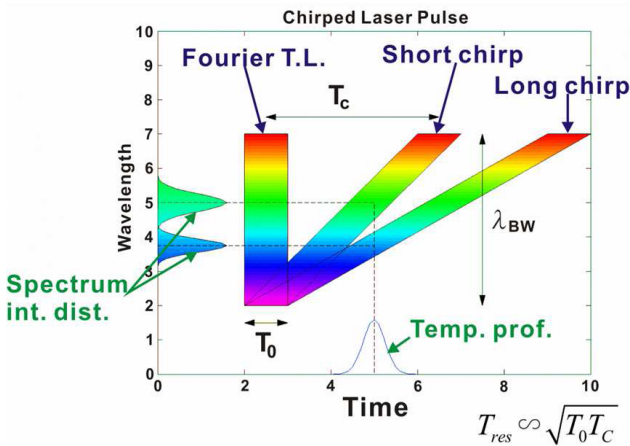
Figure 2: EO-encoded spectra with different chirp rate.
