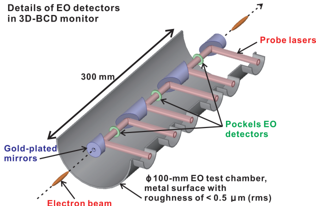
Figure 3: Schematic drawing of element of the 3D-BCD monitor ( upper ) and total system of 3D-BCD monitor ( lower )
