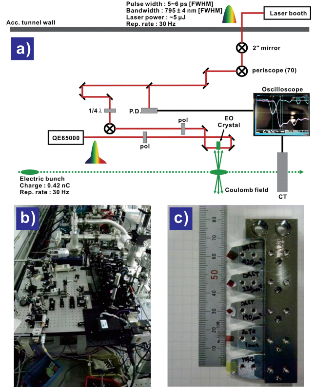
Figure 5: Experimental setups of the BCD measurement at the Prototype Test Accelerator, SPring-8 (a and b), and crystals for beam detection (c, starting from the top, 420, 230, 190 mm thick of DAST crystals, 1 mm thick ZnTe and Ce:YAG).
