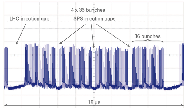
Figure 5: 10 \mu s zoom; the structure of 4x36 bunches is resolved. The LHC injection gap and the SPS injection gaps separate the bunch trains containing 36 bunches each.
