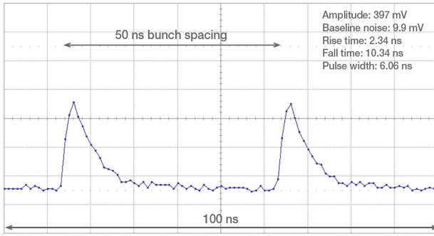
Figure 7: 100 ns zoom; single bunches are resolved with a rise time of 2.34 ns, a rms baseline noise of 9.9 mV and an amplitude of 397 mV. The corresponding intrinsic time resolution is 58 ps.
