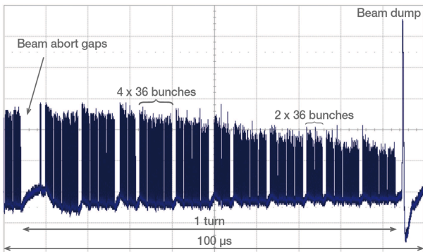
Figure 4: 100 \mu s zoom; the beam abort gap, and the bunch structure is resolved: a pattern of two 4x36 bunches and one 2x36 bunches are periodically cycling in the LHC. The losses caused by the beam abort are synchronous to the beam abort gap.
