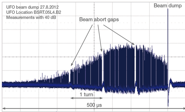
Figure 3: 500 \mu s zoom; UFO location in Point 4, recorded in the collimation area in Point 7 with a 10x10x0.5 mm 3 diamond detector with 40 dB signal amplification. The length of the loss is about 0.5 ms. Beam abort gaps are clearly resolved.
