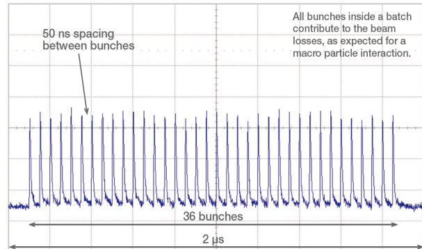
Figure 6: 2 \mu s zoom; the bunches are separated by 50 ns, 36 bunches form a batch. It is remarkable that all bunches inside a batch contribute to the beam losses, as expected for a macro-particle interaction.
