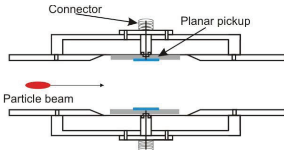
Figure 2: Cross-section of planar transmission line pick-ups for the EBPM.
