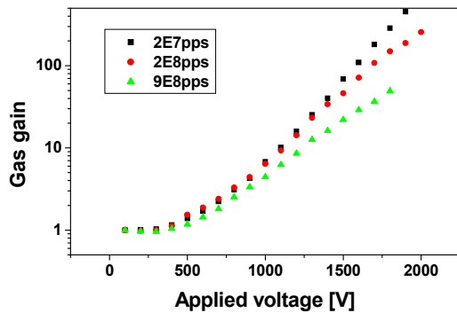
Figure 5: Measured gas gain with different beam intensities.
