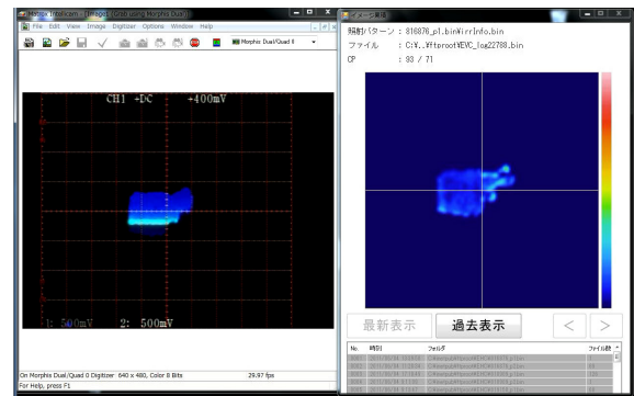
Figure 7: Online display of position monitor measurement, left: online display of beam position, right: measured fluence map for each iso-energy slice.
