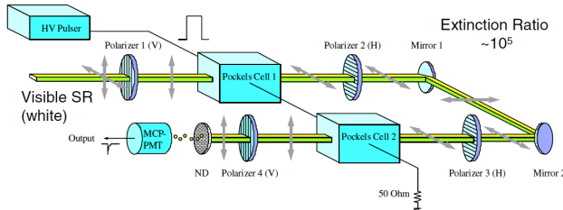
Figure 3: The schematic layout of the bunch purity monitor.
