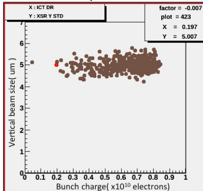
Figure 6: Vertical beam size measurement in 2012.
