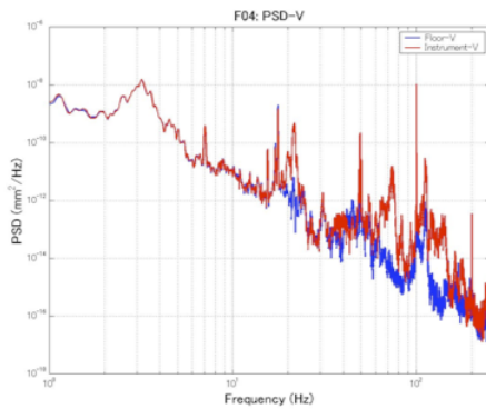
Figure 5: Spectrum of the mechanical vibration in vertical direction at the Si monochromator.
