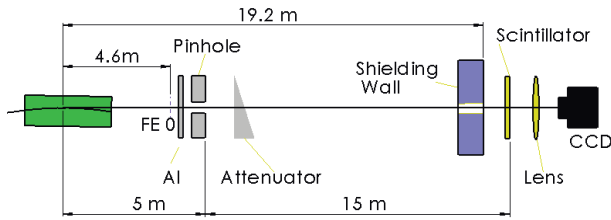
Figure 4: Layout of the X-ray pinhole camera.
