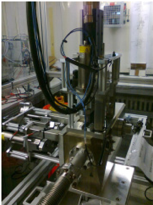
Figure 5: XFEL wire scanners' test setup
