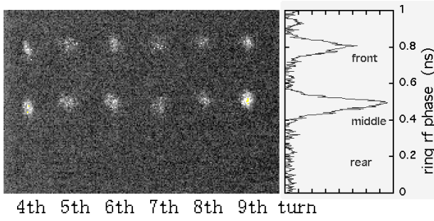
Figure 7: Dual Sweep image of the injected beam of the shot #12.
