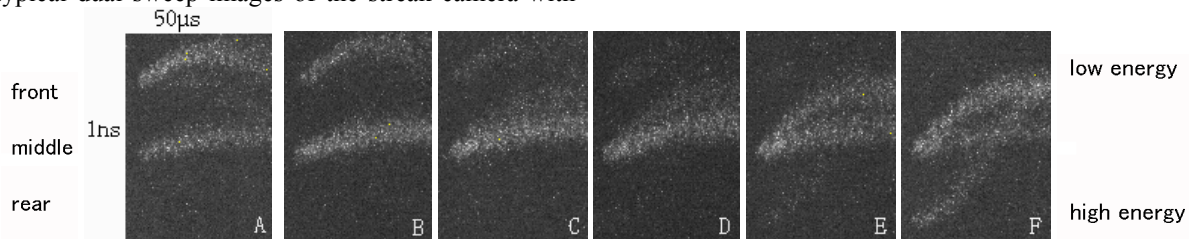
Figure 3: Typical dual sweep images. Because of the non-linear momentum compaction factor, the movement of the front bunch is slower at the initial 50 \mu s.
