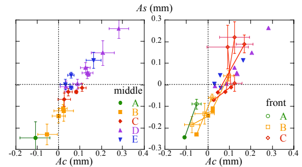
Figure 12: Shot-to-shot fluctuation of the dipole oscillation of the middle bunch (left) and those of the front bunch (right). The oscillations of different bunches in the same shot are connected with lines.
