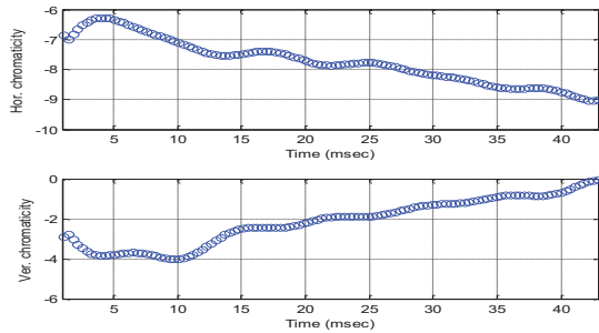
Figure 12: Measured uncompensated chromaticity.
