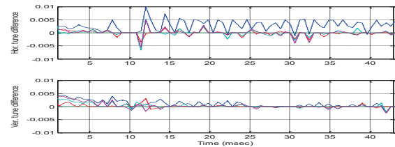
(b) Fractional tune difference.
