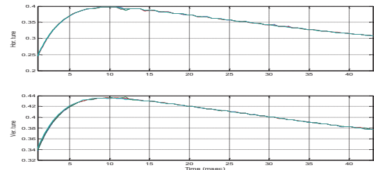
(a) Tune variation as function of ramping time.
