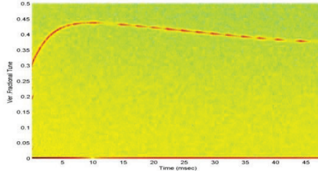
(b) Vertical tune variation during ramping cycle
