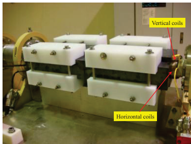
Figure 5: Magnetic shaker.
