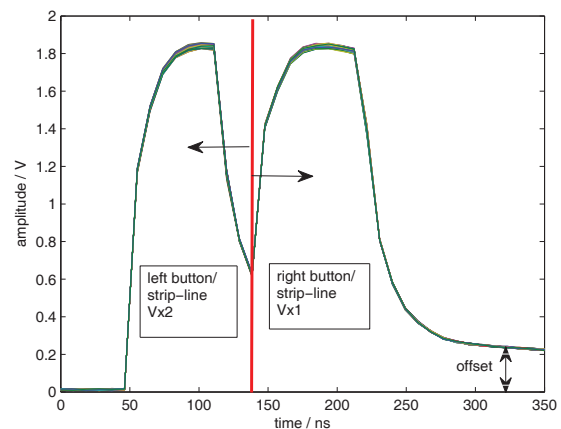
Figure 7: Raw data for a centered beam measured at 500pC for the strip-line monitor. The sampling time step is 9.23ns. The data is taken for 100 subsequent pulses in single-bunch mode.
