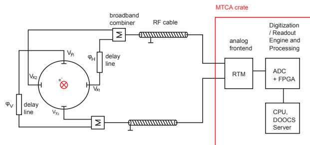
Figure 1: BPM conceptual system setup. One signal of each plane from the BPM is combined with the other after a delay of ca. 100ns. The combined signals are then transported over a long RF cable from the tunnel to the electronic racks.
