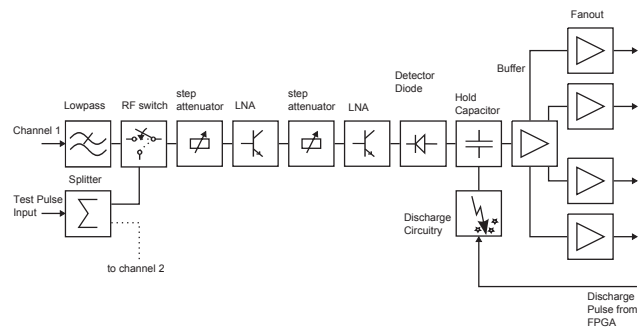
Figure 5: Block diagram of the front-end for the position measurement in one plane.
