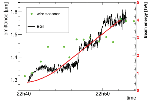
Figure 7: Emittance behaviour during ramp.
