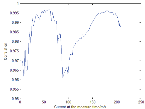
Figure 6: Evaluation by correlation.
