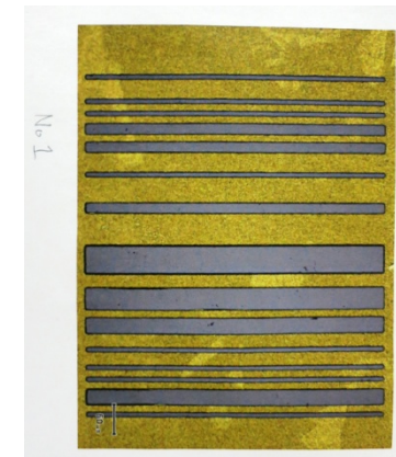
Diamond+Au mask Minimum slit width 10 \mu m
