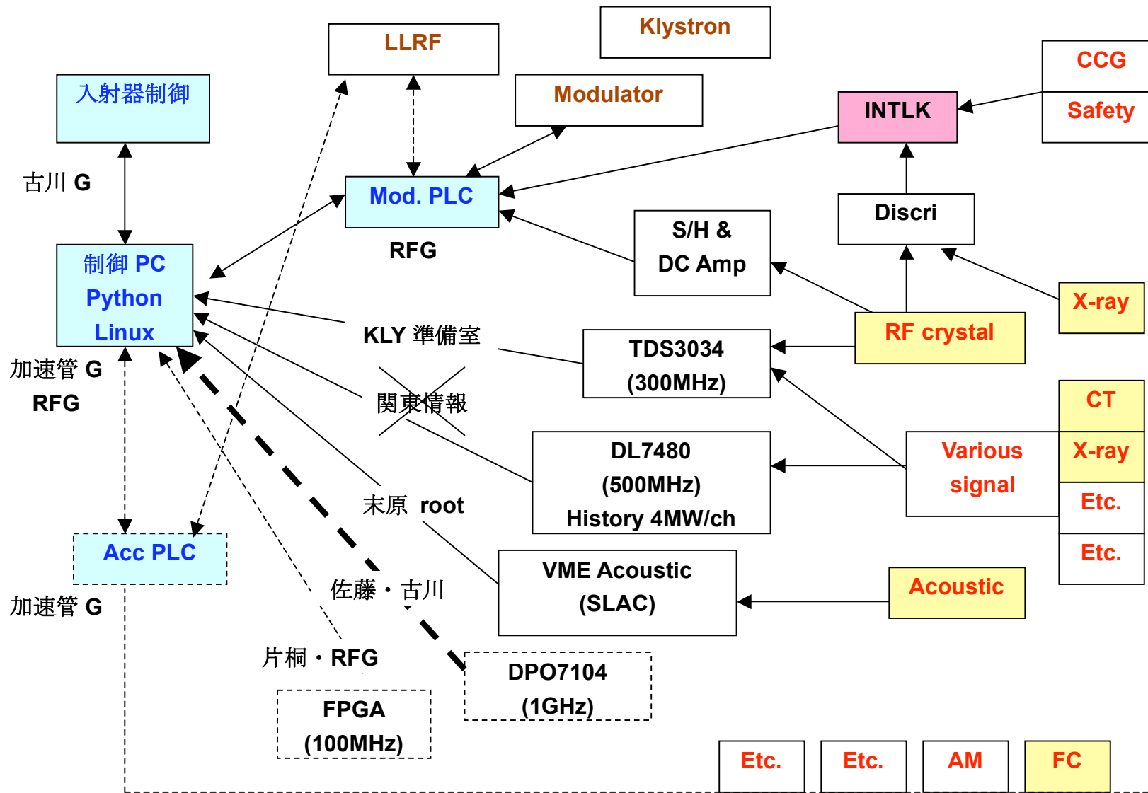
New XTF at Acc Structure Assembly Room at KEKB Injector (plan 070410)
