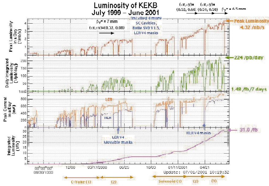
Figure 1: History of the KEKB luminosity.
