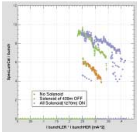
Figure 2: Effect of solenoid magnets on the luminosity.
