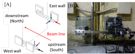
Figure 6: The installation situation of dial gauge at 2-8.
