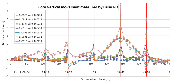
Figure 3: Vertical laser PD measurement with respect to 20140731.
