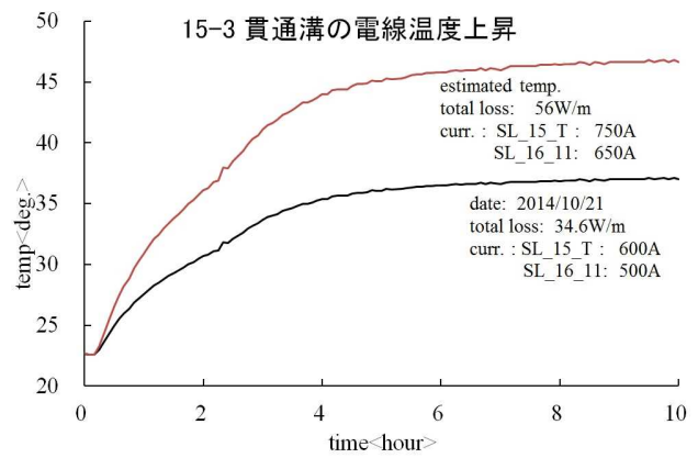
Figure 3: Cable temperature through the duct.
