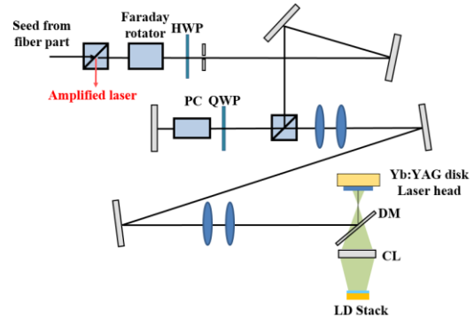
Figure 7: Regenerative amplifier cavity configuration.
