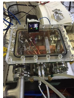
Figure 4: low temperature laser vacuum chamber.
