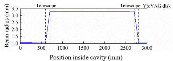
Figure 8: Beam radii in cavity shown in Figure 7.
