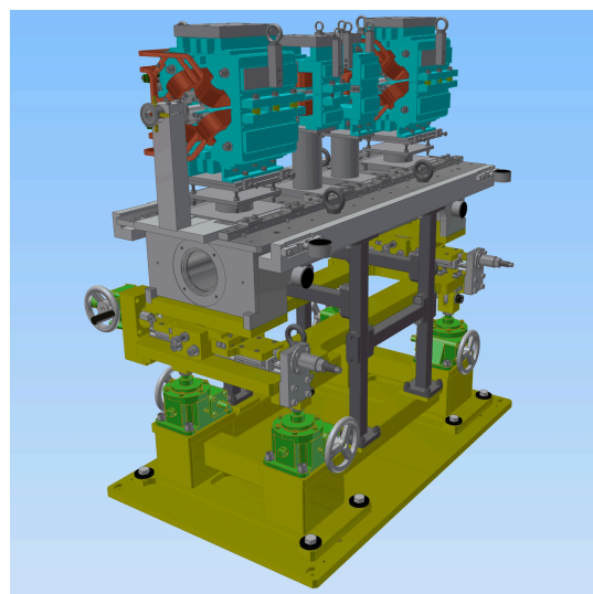
Figure 4: Girder design with precise alignment movers.
