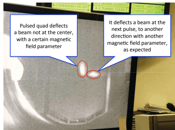
Figure 3: The beam test of pulsed magnets with pulse-to-pulse beam displacements.
