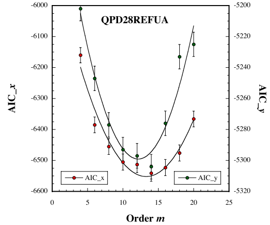
Figure 3: Variations in (a) the x and (b) y AICs calculated for QPD28REFUA as a function of the order m in a linear-regression analysis.
