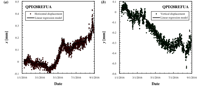
Figure 2: Time traces of (a) the horizontal ( x ) and (b) vertical ( y ) displacements of QPD28REFUA during the term Jan.07-Aug.26.2016.
