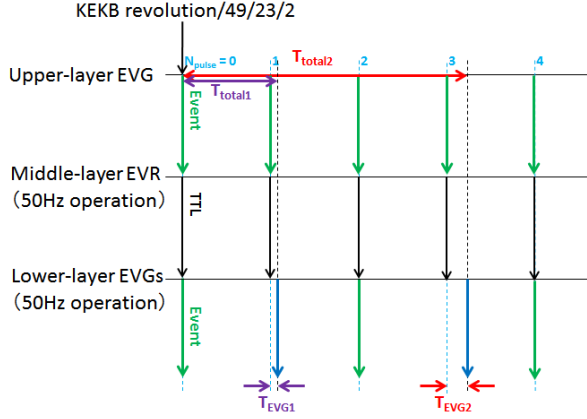
Figure 3: The schematic view of timing determination for the LER injection: it explains in the case injecting positrons into DR at pulse #1 and extracting them at pulse #3. Two black dashed lines show the operation timings of injection and extraction. The T_{total1} and T_{total2} are determined as the interval from the input trigger of upper-layer EVG while the T_{EVG1} and T_{EVG2} are determined as the interval from the individual output triggers of upper-layer EVG.
