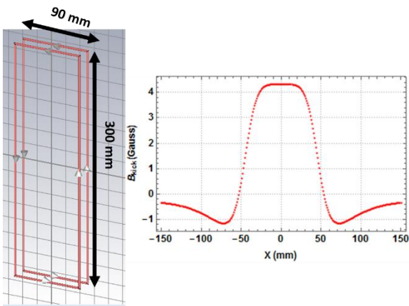
Figure 10: (Left) Rectangular dipole kicker coil design in CST the size (width) of the coil correspond to \pi/6 shape. Right: Field profile of kicker coil in the X (mm) direction.
