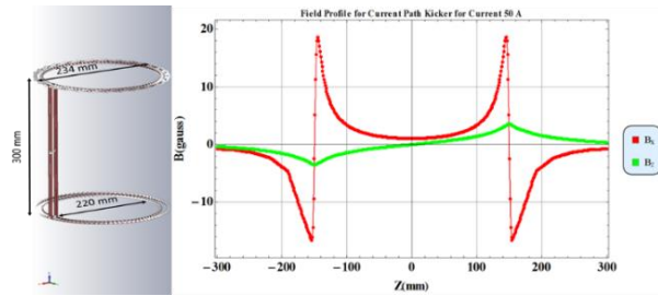
Figure 9: (Left) The model of kicker coils to produce uniform 2\pi kick. The direction of the current in upper and lower coils are opposite to each other. These pairs of coils produced cylindrical symmetric field. Right: Field profile of kicker coil along the axial direction.
