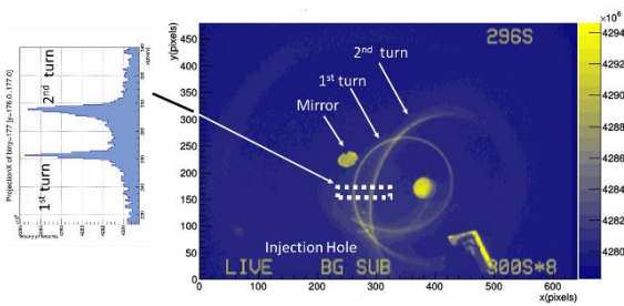
Figure 2: The electron beam spiral trajectory as a visible light due to the de-excitation of the nitrogen gas in the storage magnet vacuum chamber.
