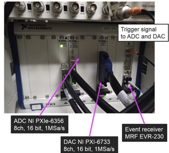
Figure 4: Details of the PXI unit (top) and its outlook (bottom).
