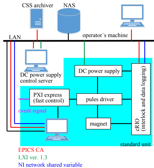
Figure 2: Block diagram of the power supply control and monitor system.
