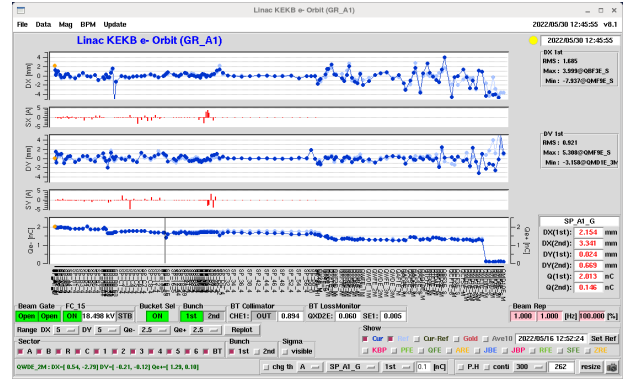
Figure 5: Current electron beam orbit.
