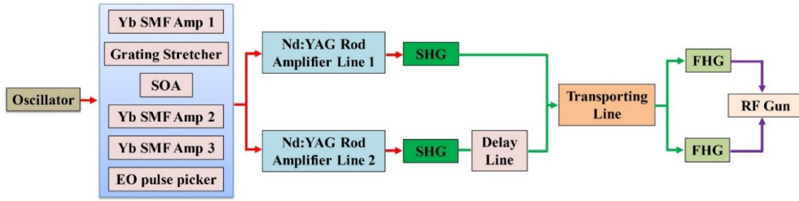
Figure 1: The layout of current Yb/Nd hybrid laser system for SuperKEKB commissioning.
