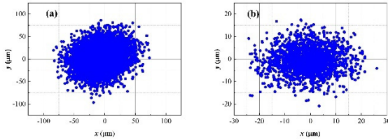
Figure 4: One-day position records of the UV laser beam at virtual photocathode position without and with laser position sensor and feedback system.
