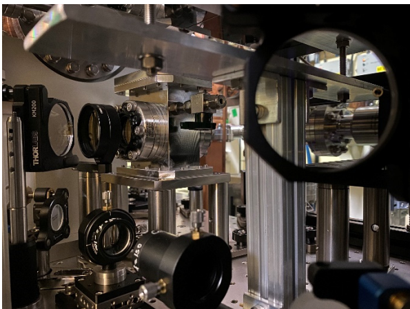
Figure 2: The DOE chamber in the 2nd laser line.
