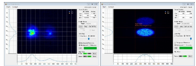
Figure 3: The UV laser beam spatial distributions without and with the application of DOE.
