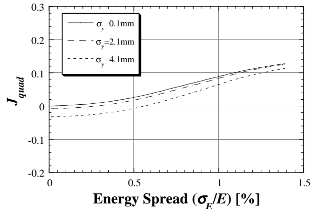
Figure 4: Variation of the quadrupole moment to the energy spread expected at the 180-degree arc.
