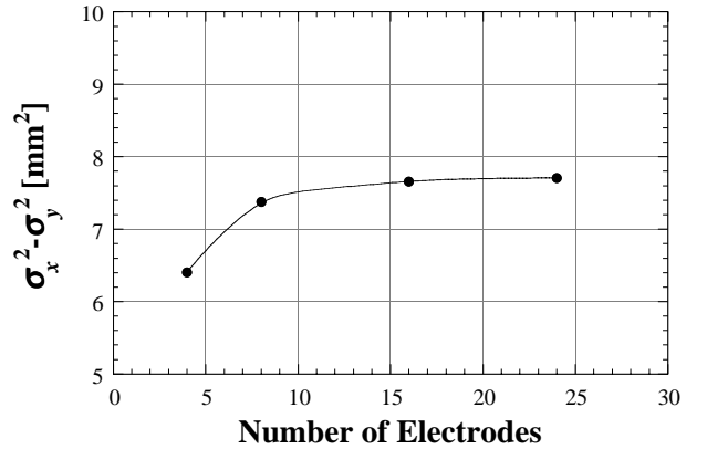
Figure 3: Variation of the square difference of the beam sizes depending upon the number of electrodes. The horizontal and vertical beam sizes are assumed to be \sigma_x = 3 mm and \sigma_y = 1 mm, respectively.
