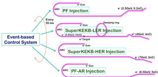
Figure 4: Single injector linac behaves as four PPM virtual accelerators, being managed by an event-based control system.
