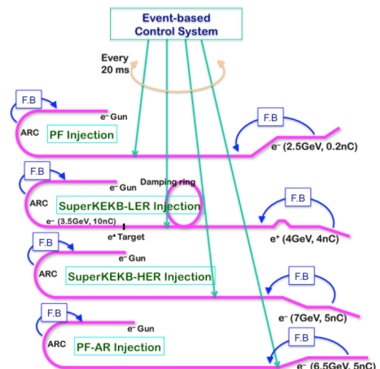
Figure 5: Each of multiple virtual accelerators may be managed by several stabilization feedback loops.
