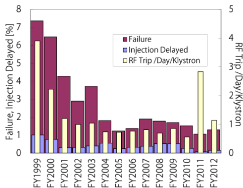
Figure 3: Failure, Injection delay rate and RF trip.
