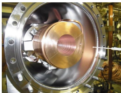
Figure 6: Flux Concentrator.
