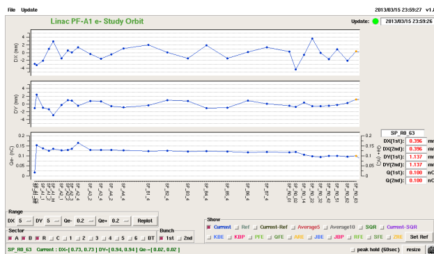
Figure 5: Beam Position and Charge.
