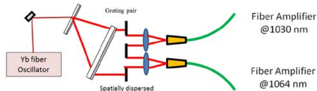
Figure 6: Spectrum separation by grating pair.
