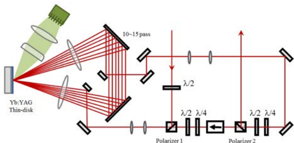
Figure 4: Thin-disk multi-pass amplifier with cavity.
