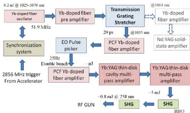
Figure 1: Layout of Laser system.
