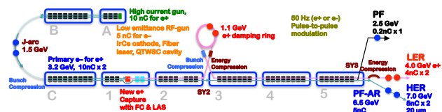
Figure 1: Injector linac layout and beam delivery to multiple experimental facilities.
