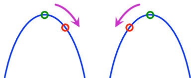
Figure 3: Energy knob to adjust energy from crest phases (green) to operation phases (red) compensating energy spread.
