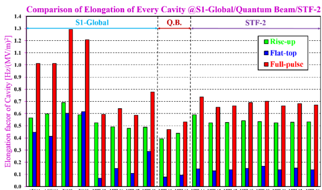
Figure 4: Comparison of the LFD for the S1-Global (w/ four TESLA cavities), the capture (named the Quantum Beam cryomodule in 2012), and the STF-2 cryomodules.
