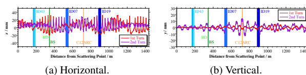
(a) Horizontal. (b) Vertical. Figure 11: Trajectory in 1st turn and the 2nd of scattered particle at C36 Arc with momentum deviation 4.6 %.
