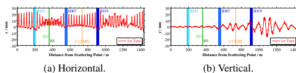
(a) Horizontal. (b) Vertical. Figure 10: Trajectory in 1st turn of scattered particle at C36 SS with momentum deviation 5.4 %.
