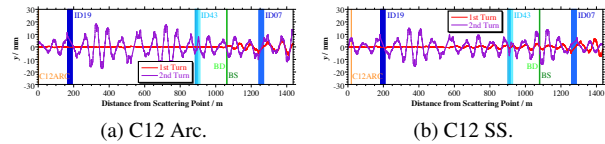
Figure 15: Vertical trajectory in 1st turn and the 2nd of scattered particle at C12 Arc (SS) with momentum deviation 4.6 % (5.4 %).
