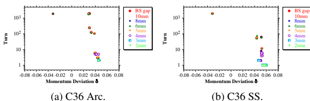
(a) C36 Arc. (b) C36 SS. Figure 9: Simulated \delta -Turn distribution of Tauschek loss on ID19.
