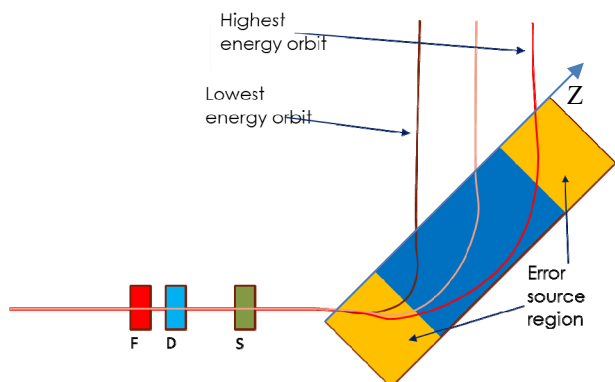
Figure 6: Beam orbits and bending magnet with field shoulder in the Z direction.
