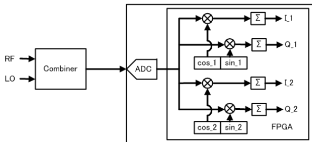
Figure 6: Experimental setup of RF-LO simultaneous measurement under RF-LO combined signal.
