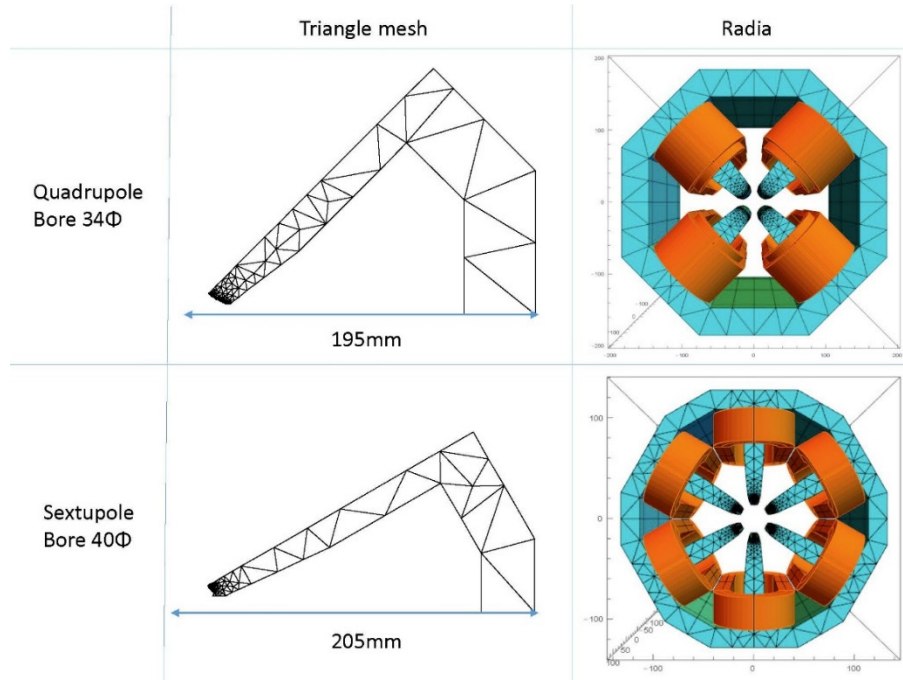
Figure 5: Mesh diagrams used for Radia computations of SLiT-J quadrupole (top middle) and sextupole (bottom middle) magnets. Quadrupole (top right) and sextupole (bottom right) magnet 3D models for Radia computations.
