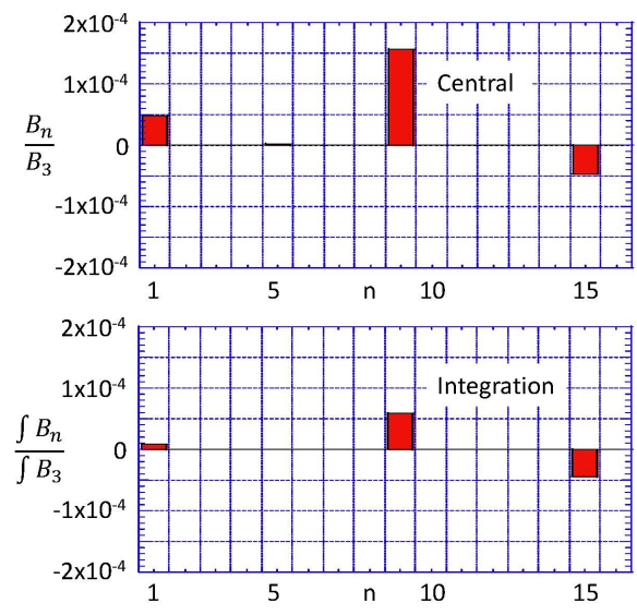
Figure 9: Ratio of multipole fields to sextupole magnet fields at x = 0.01\text{m} .
