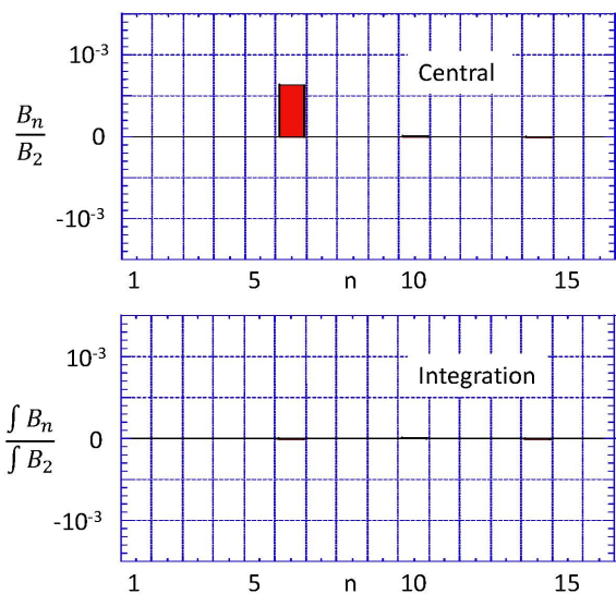
Figure 7: Ratio of multipole fields to quadrupole magnet fields at x = 0.01\text{m} .
