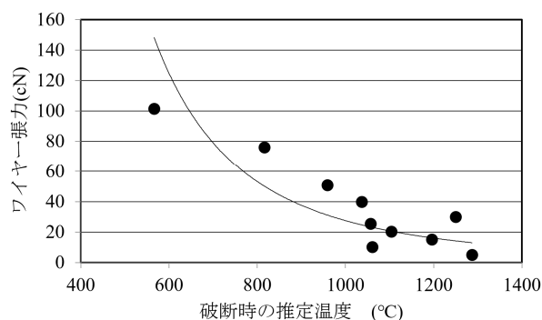
Figure 7: Tensile fracture strength of \phi 20 \mu\text{m} wire with estimated Temperature.
