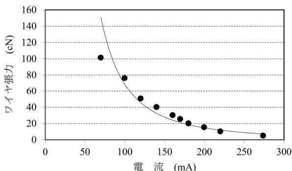
Figure 6: Tensile fracture strength of \phi 20 \mu\text{m} wire with electrical current.
