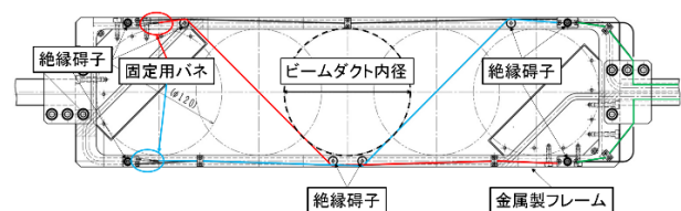
Figure 1: A WSM-sensor head and wires employed at beam lines in J-PARC linac. Red and blue lines are metallic wire mounted on a frame with ceramic insulators. Green lines are insulated cable.
