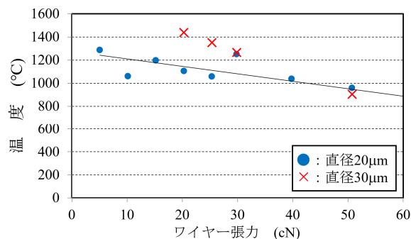
Figure 8: Tensile fracture strength of \phi 20 \mu\text{m} and \phi 30 \mu\text{m} wire with estimated temperature.
