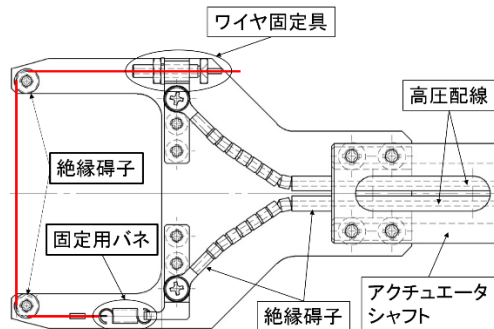
Figure 2: A BSM head to generate and accelerate secondary electrons. Red line is a metallic wire mounted on a frame with a spring for the tension control.
