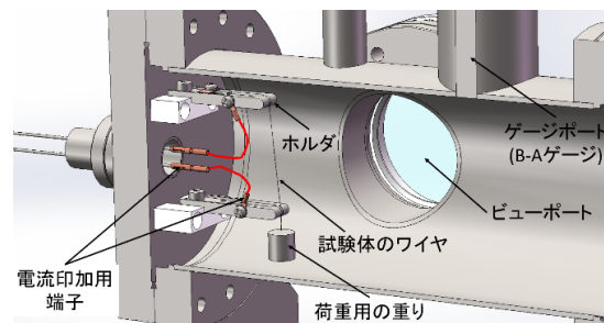
Figure 4: Inside structure of vacuum chamber.
