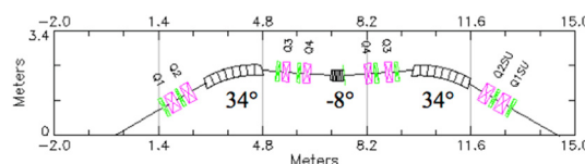
Figure 2: Geometrical plot of magnets per cell in NewSUBARU. The cell is composed from two 34 degrees bends and one -8 degrees inversely bending magnet.
