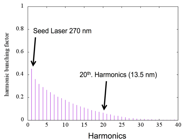
Figure 11: Harmonic bunching factor of PEHG process in the case of NewSUBARU-2.0. If the seed laser wavelength is 270 nm, the 20 th harmonics corresponds to 13.5 nm that is needed for the EUV lithography.
