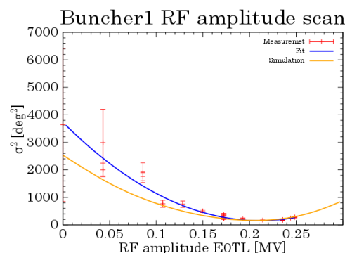
Figure 6: First measurement of BSM in MEBT1.
