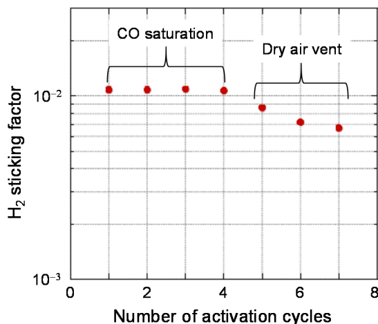
Figure 7: Change of H 2 sticking factor as a function of number of activation cycles.
