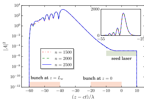
Figure 3: Temporal shapes of FEL pulses in a perfectly synchronized optical cavity with an external seed laser after 1500, 2000 and 2500 round trips.
