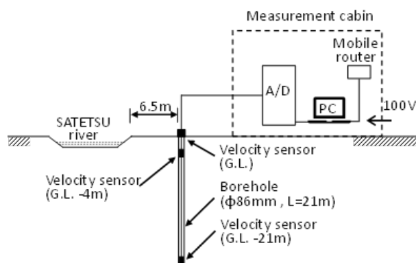
Figure 2: Measurement system.
