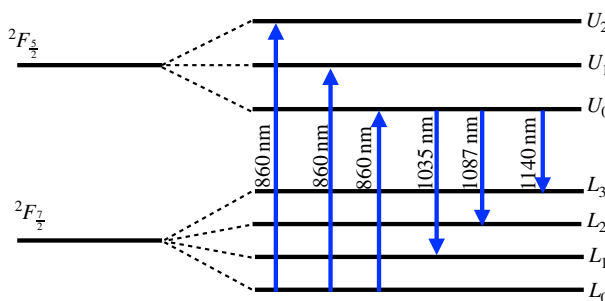
Figure 4: Energy level structure of Yb silica glass.
