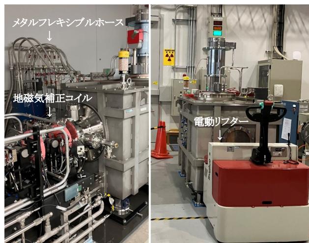
Figure 3: SACLA electron gun and the electric lifter.
