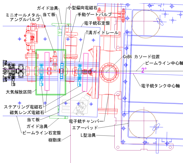
Figure 1: Layout of the modified SACLA electron gun.
