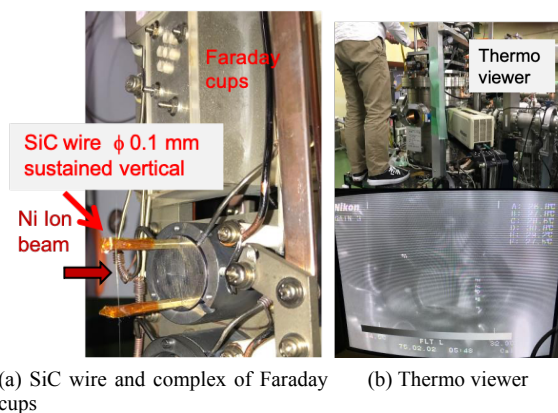
Figure 5: Experimental setup at TIARA for Ni beam, (a) SiC wire and Faraday cups to observe the beam current, (b) Thermo viewer to observe the temperature of the sample.
