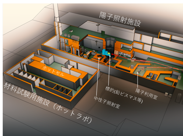
Figure 1: View of the proton beam irradiation.
