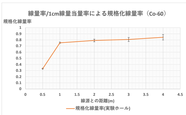
Figure 4: Variations in the dose rate normalized by 1cm-equivalent dose rate as a function of the distance measured in the irradiation facility.
