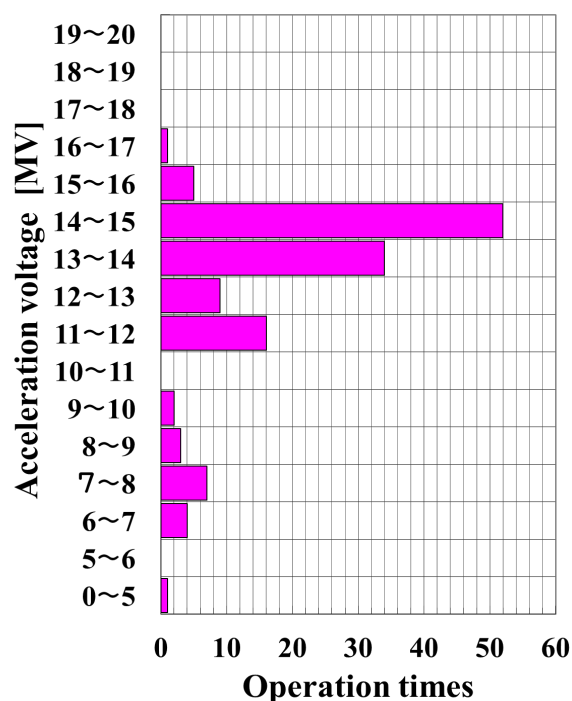
Figure 6: Distribution of acceleration voltages for experiment in FY2023.
