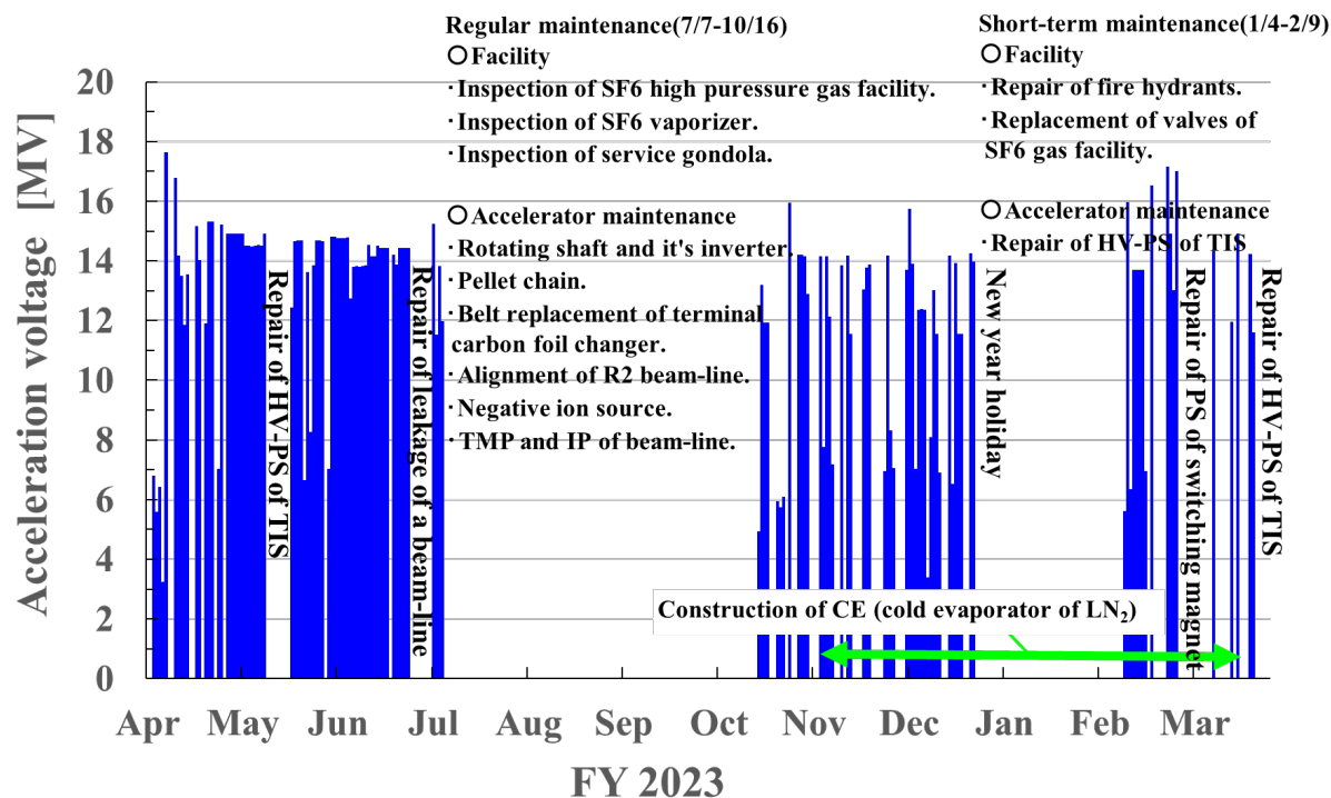
Figure 1: Daily accelerating voltage and operation status in the FY 2023.
