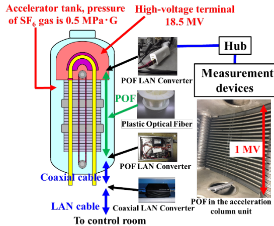
Figure 9: Schematic diagram of the LAN system in the tandem accelerator tank.
