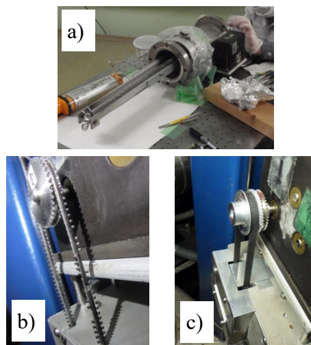
Figure 8: a) Photo of carbon foil changer for electron stripper in high-voltage terminal. b) Broken belt (NO-SLIP POSITIONING BELT). c) Glued new pulleys and new belt.
