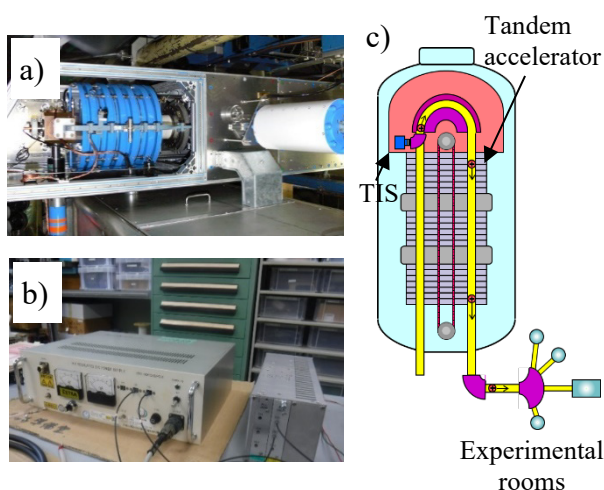
Figure 7: a) Photo of TIS (Terminal ECR Ion Source). b) Operation test of the high-voltage power supply. c) Diagram of TIS installation in high-voltage terminal.
