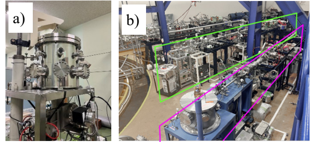
Figure 10: a) The vacuum chamber for irradiation of space equipment. b) Two beamlines to be installed.
