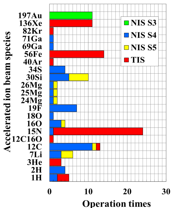
Figure 5: Distribution of accelerated ion beams species for experiment in FY2023.
