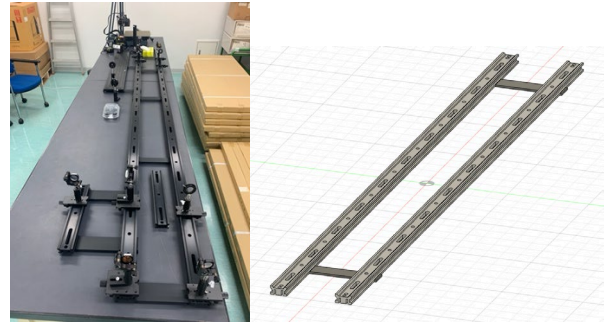
Figure 4: A photo drawing a part of the pilot harmonic resonators.
