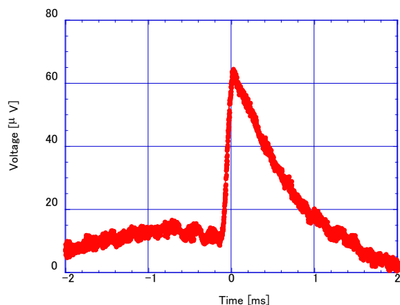
Figure 11: The voltage waveform during cable motion.
