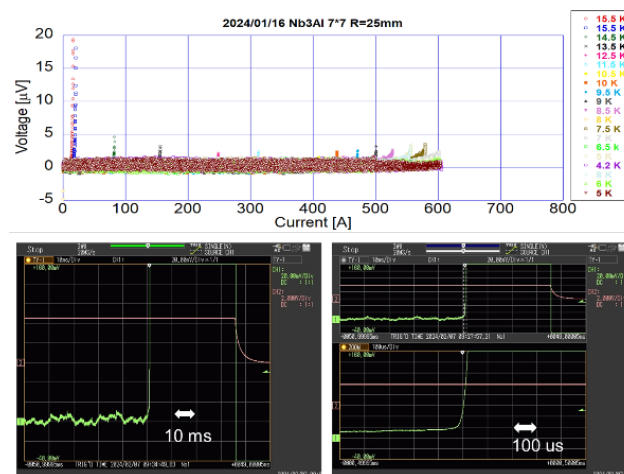
Figure 7: Variation of the voltage on a both side sample. (Upper) Change in voltage with respect to applied current. (Bottom) Change in the voltage at the quench.
