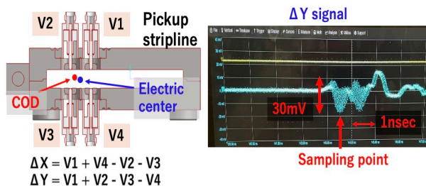
Figure 5: Schematic view of the stripline pickup (left). Beam excitation \Delta Y signal (right).
