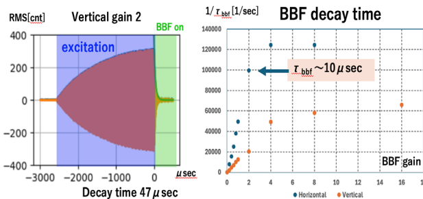
Figure 6: BBF grow damp plot (left). BBF decay time distribution depending on the BBF gain (right).
