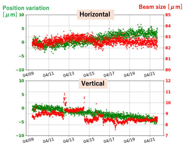
Figure 8: Stability of beam size and position variation measured using XPC in the first user operation period.
