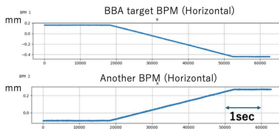
Figure 2: COD variation when stored beam orbit was changed by the steering magnet.
