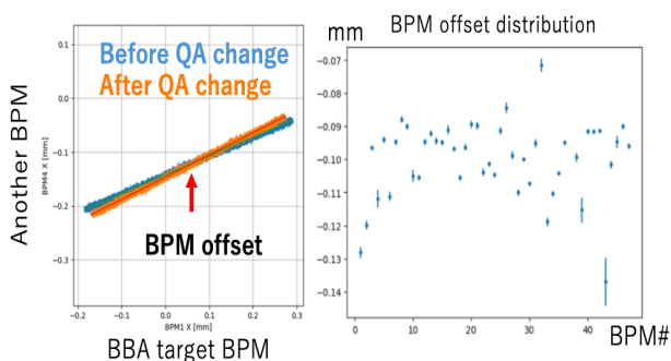
Figure 3: COD correlation plot of 2 BPMs before and after QA change (left). BPM offset distribution obtained from the intersection points with the other 47 BPMs (right).
