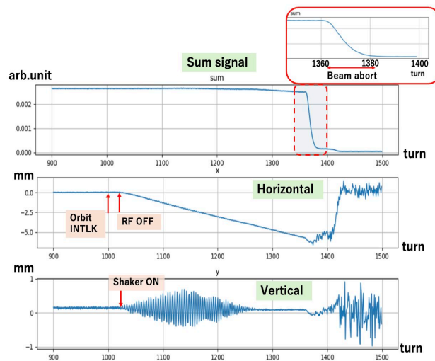
Figure 7: Single pass BPM data when the orbit interlock was triggered.
