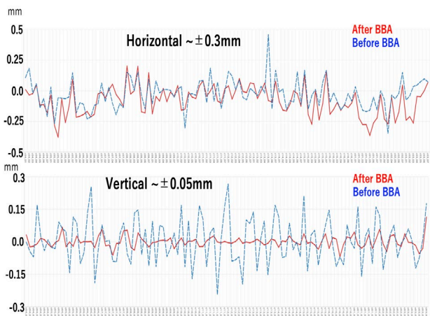
Figure 4: Horizontal and Vertical COD distribution before and after BBA correction.
