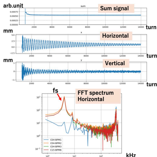
Figure 1: Single-pass BPM data and Fourier transformed spectrum. The BPM 2, 3 and 6 were installed at an energy-dispersive section. The BPM 1 was installed at a non-dispersive section.
